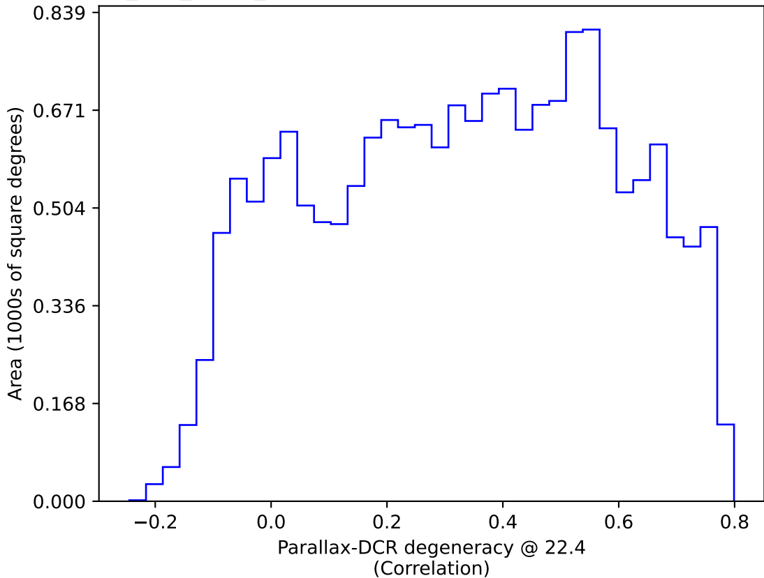
too_100_4v3.4_10yrs WFD: Parallax-DCR degeneracy @ 22.4
