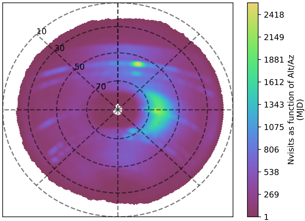
too_100_4v3.4_10yrs z band: Nvisits as function of Alt/Az
