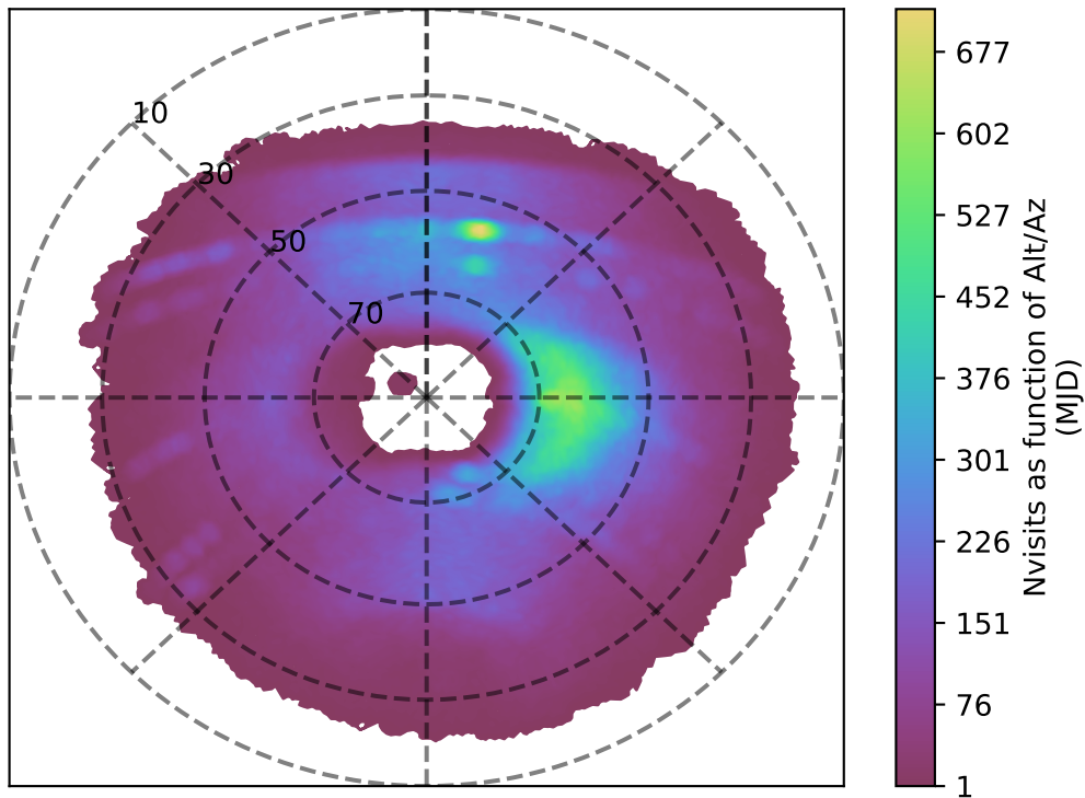
too_100_4v3.4_10yrs u band: Nvisits as function of Alt/Az
