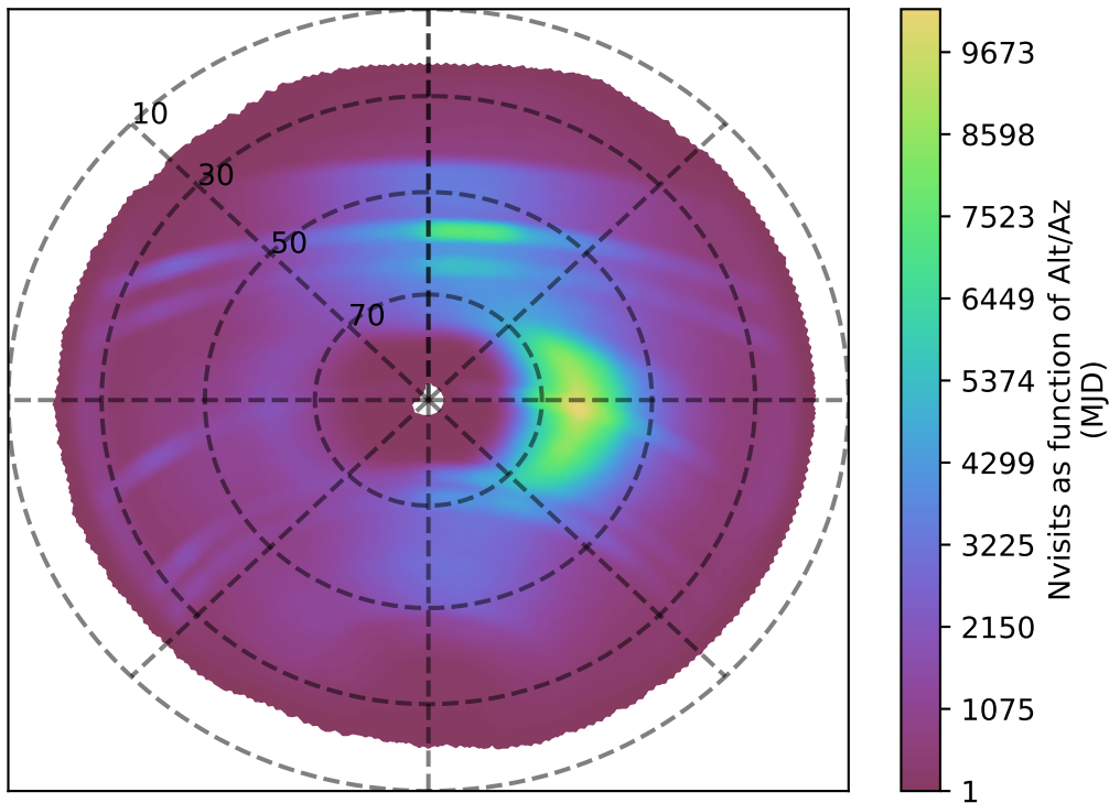
too_100_4v3.4_10yrs all bands: Nvisits as function of Alt/Az
