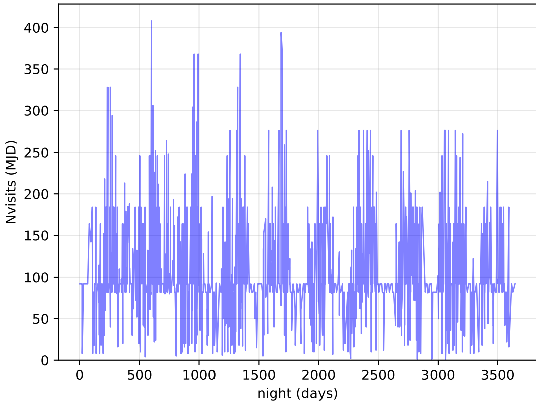
too_100_4v3.4_10yrs DDF: Nvisits
