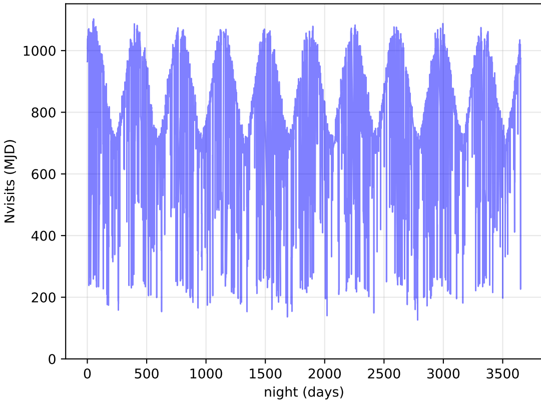
too_100_4v3.4_10yrs All visits: Nvisits
