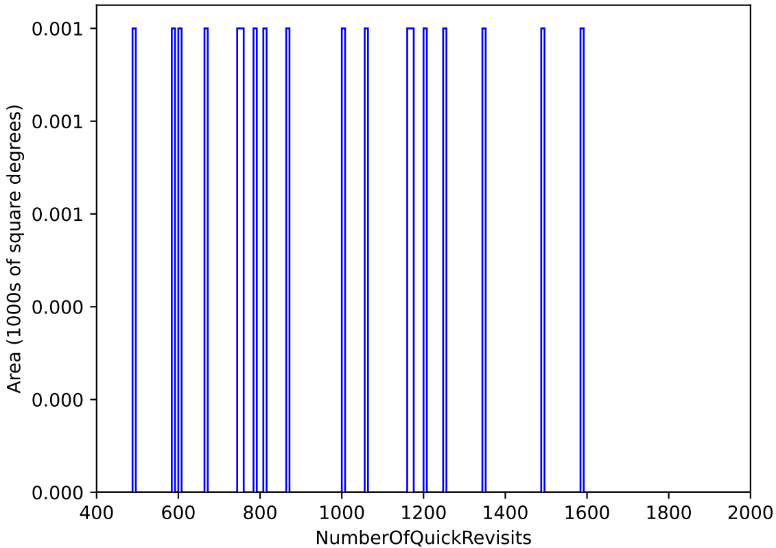
too_100_4v3.4_10yrs WFD: NumberOfQuickRevisits
