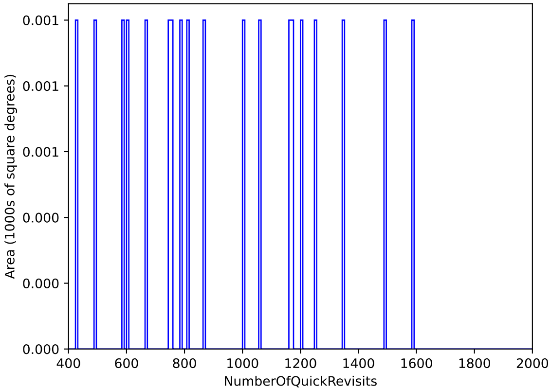
too_100_4v3.4_10yrs All sky: NumberOfQuickRevisits
