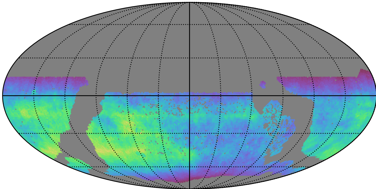
too_100_4v3.4_10yrs WFD z band: Normalized Teff
