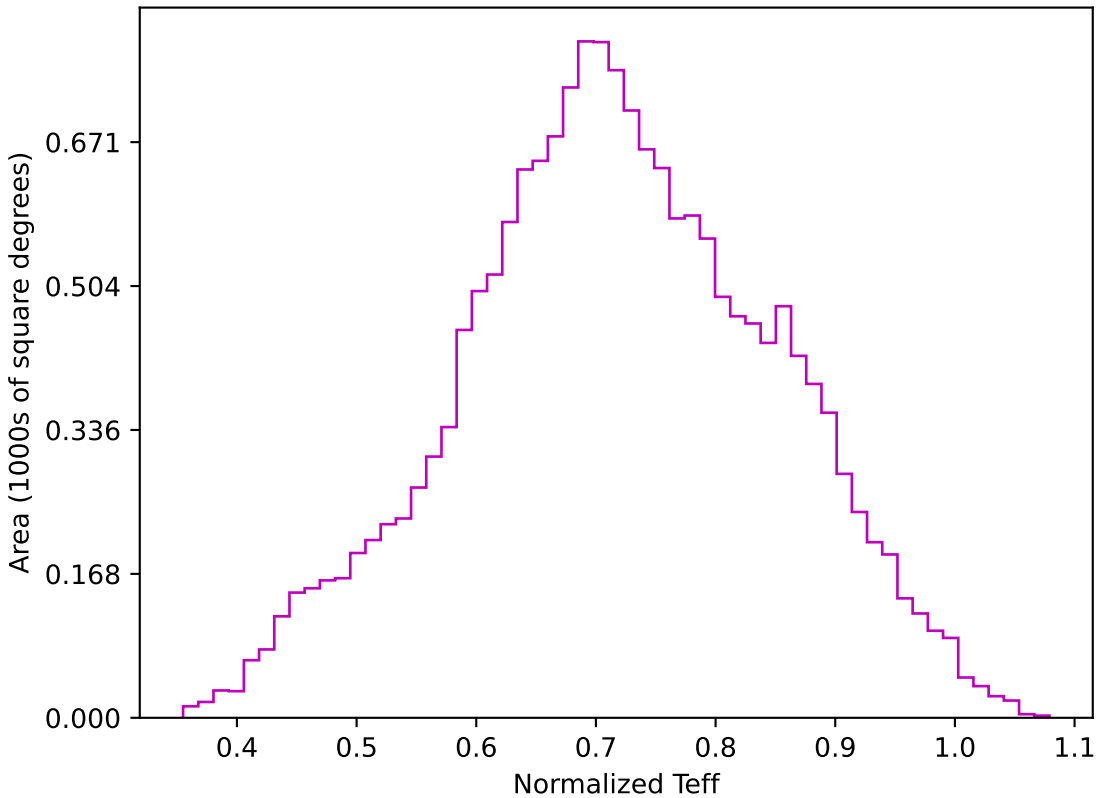
too_100_4v3.4_10yrs WFD z band: Normalized Teff
