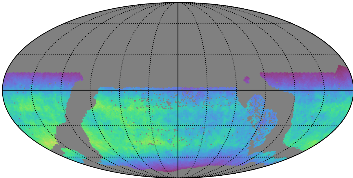
too_100_4v3.4_10yrs WFD y band: Normalized Teff
