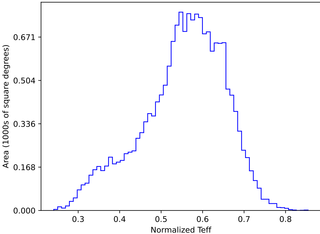
too_100_4v3.4_10yrs WFD y band: Normalized Teff
