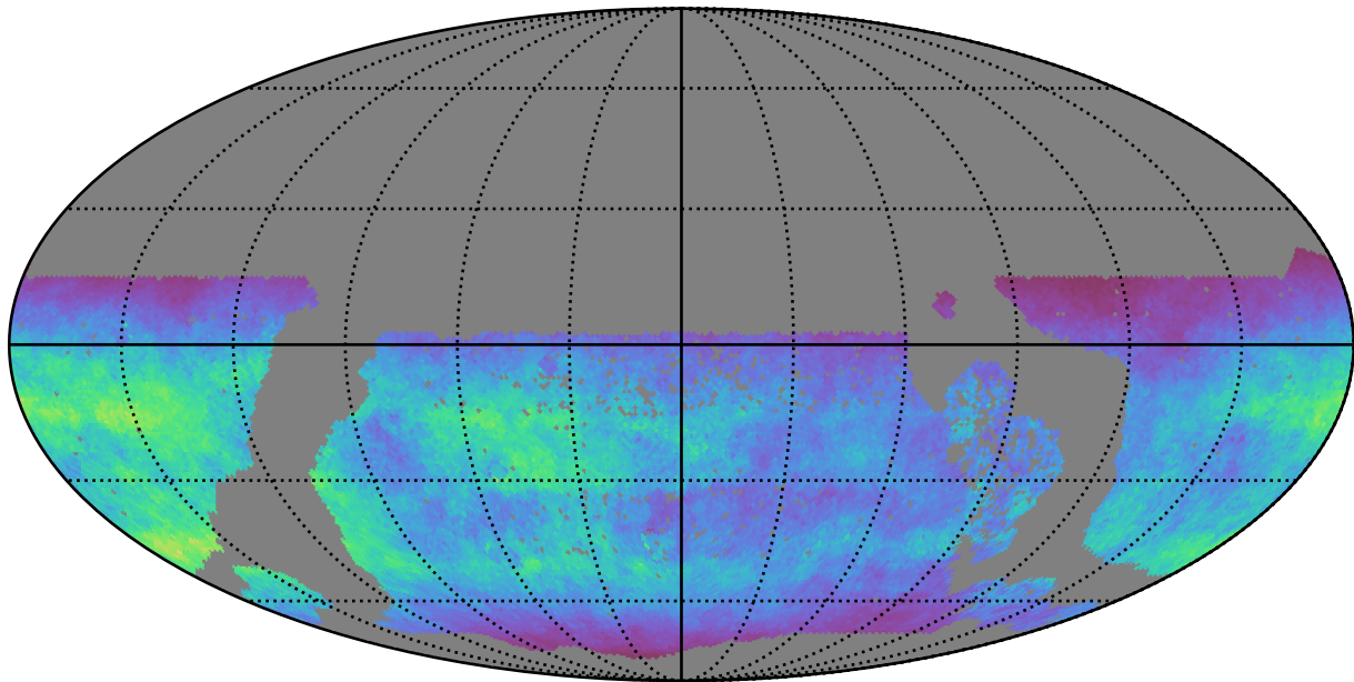
too_100_4v3.4_10yrs WFD u band: Normalized Teff
