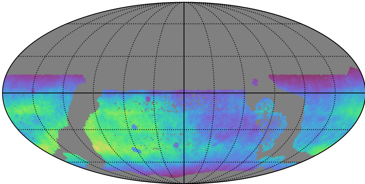
too_100_4v3.4_10yrs WFD r band: Normalized Teff
