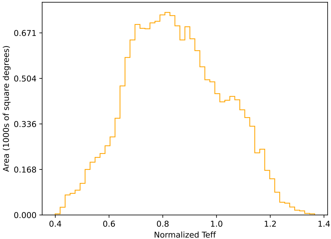
too_100_4v3.4_10yrs WFD r band: Normalized Teff
