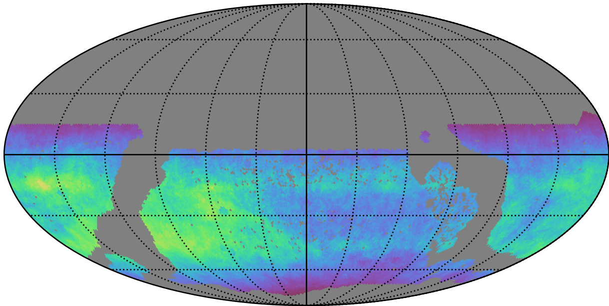
too_100_4v3.4_10yrs WFD i band: Normalized Teff
