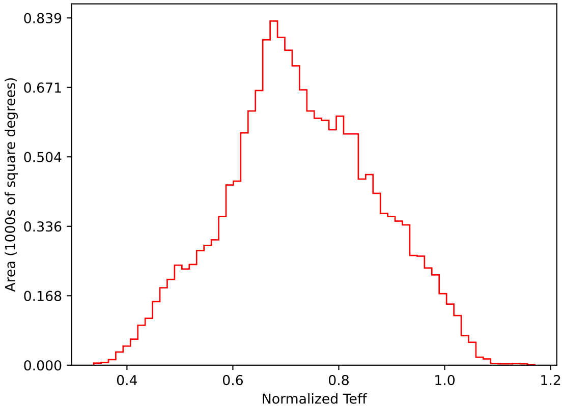
too_100_4v3.4_10yrs WFD i band: Normalized Teff
