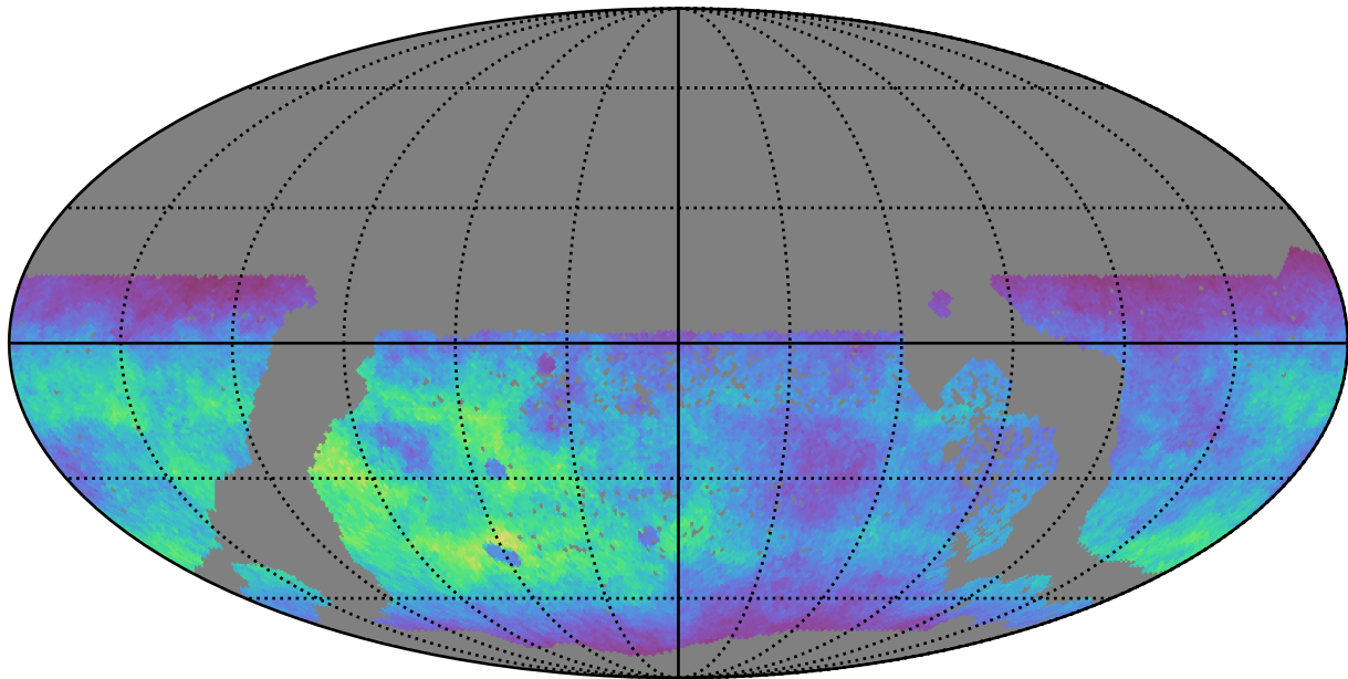
too_100_4v3.4_10yrs WFD g band: Normalized Teff
