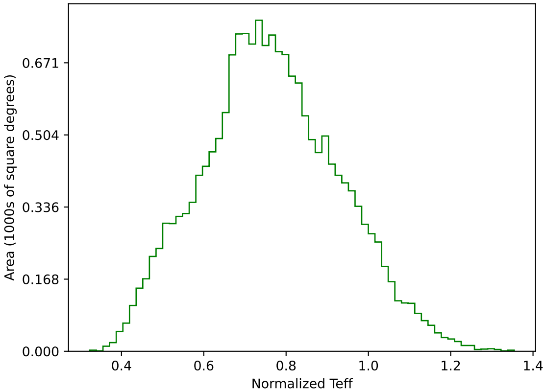
too_100_4v3.4_10yrs WFD g band: Normalized Teff
