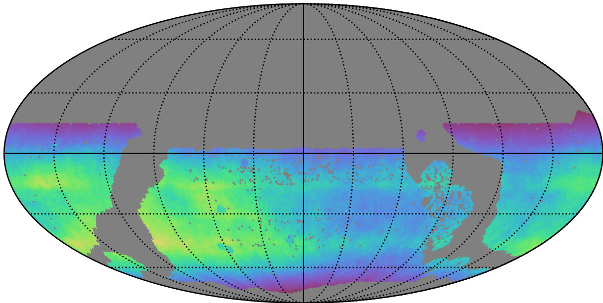
too_100_4v3.4_10yrs WFD all bands: Normalized Teff
