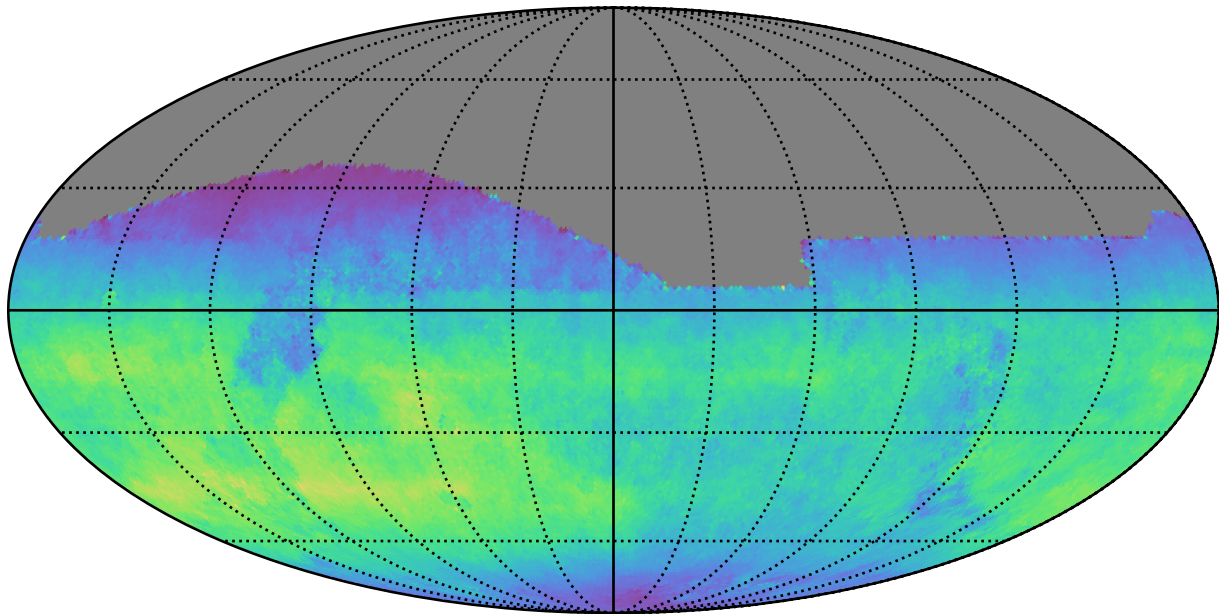
too_100_4v3.4_10yrs All sky z band: Normalized Teff
