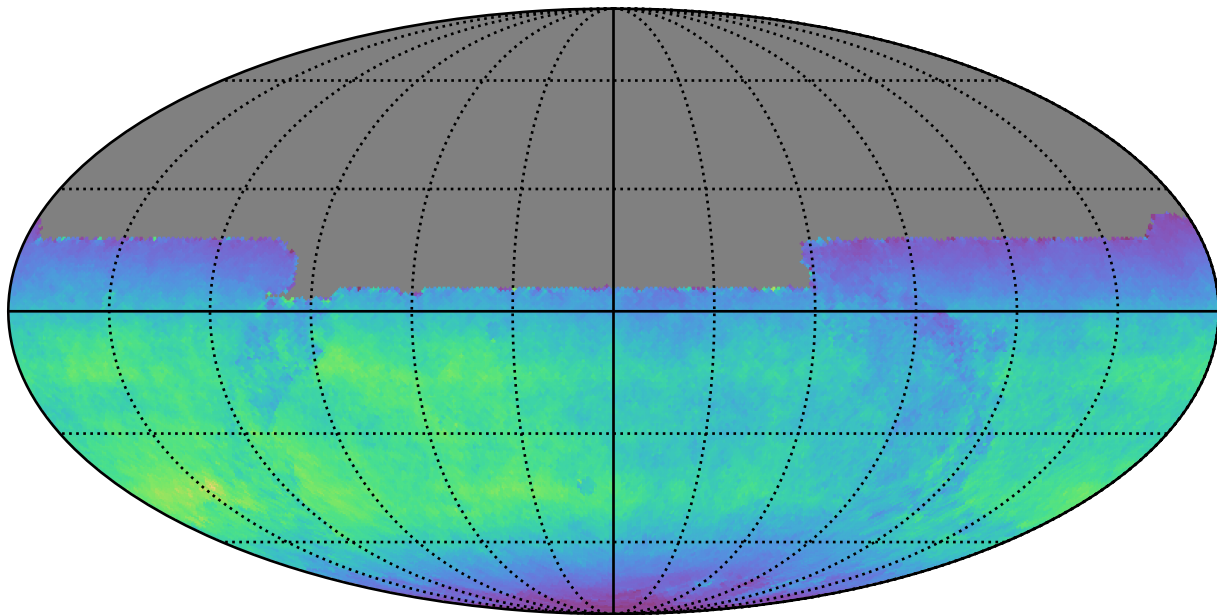
too_100_4v3.4_10yrs All sky y band: Normalized Teff
