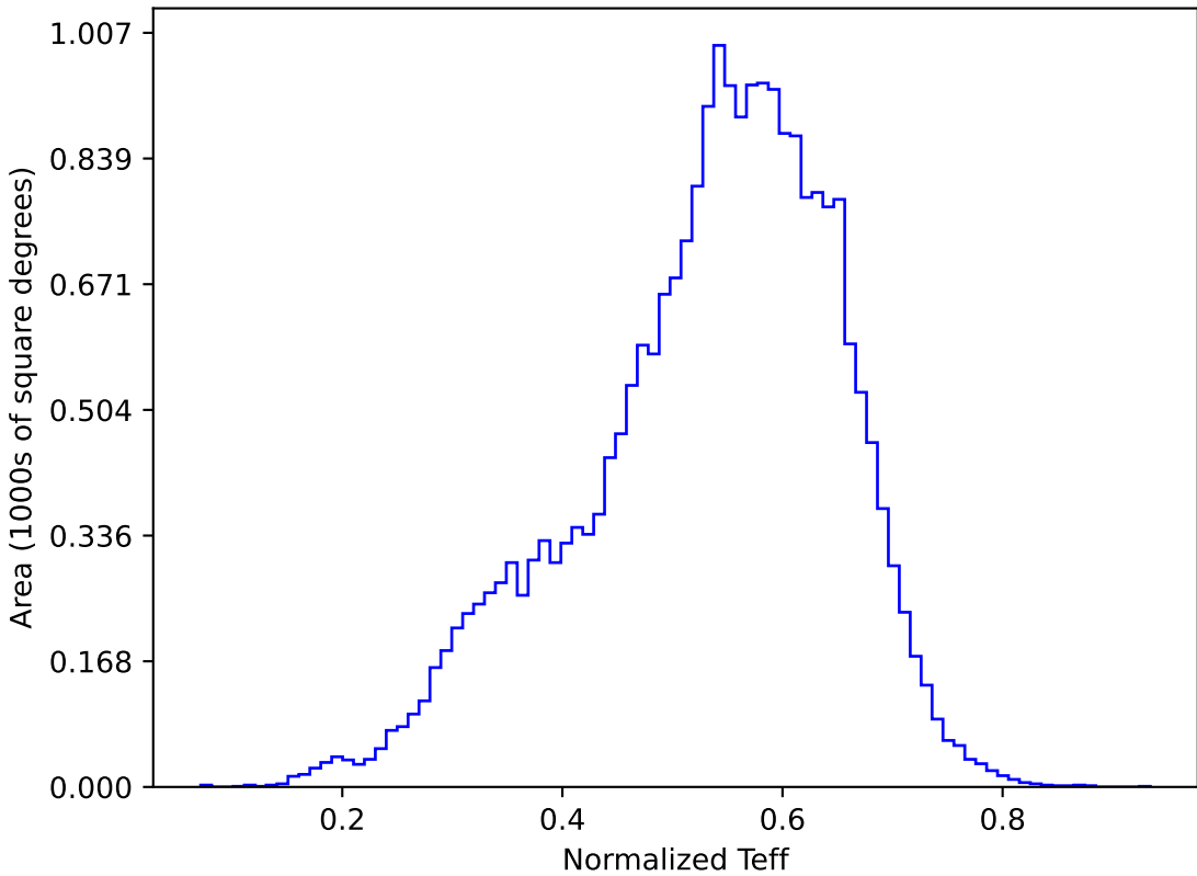
too_100_4v3.4_10yrs All sky y band: Normalized Teff
