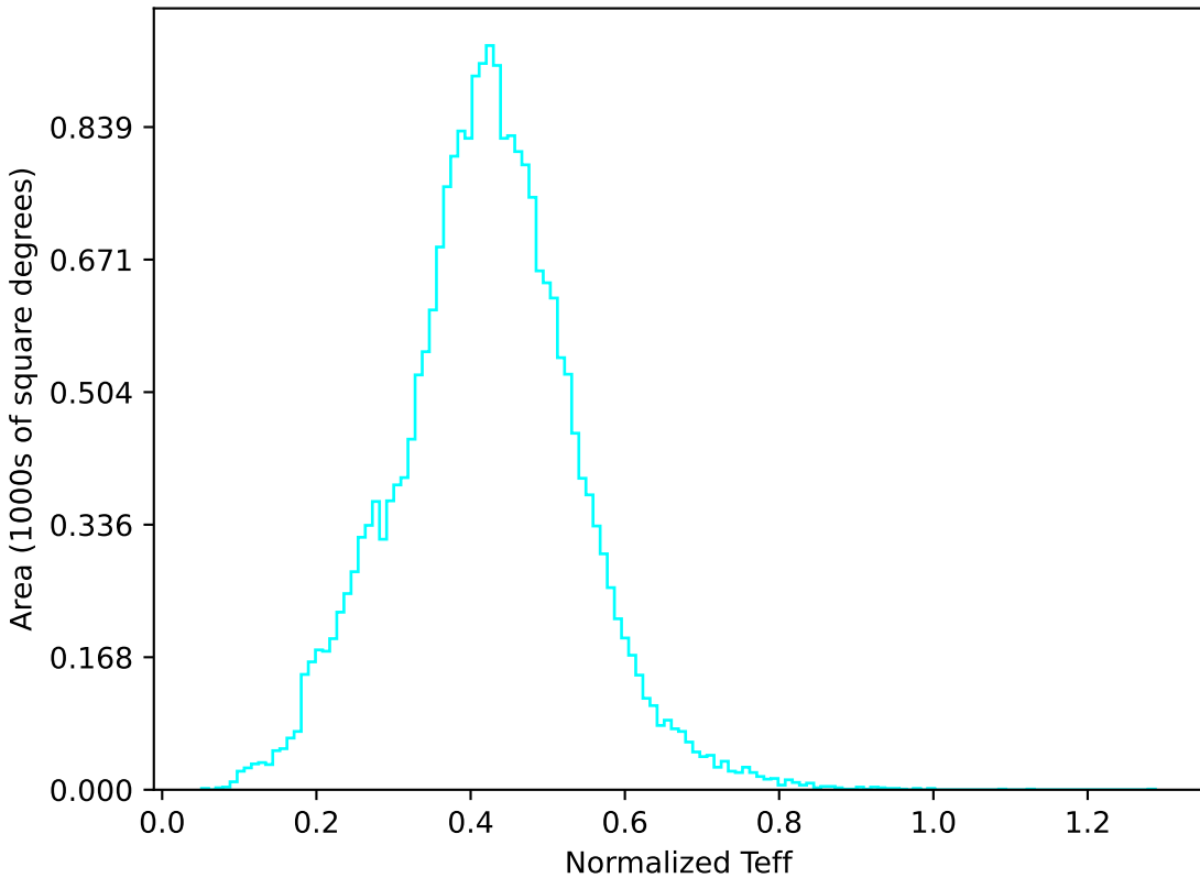
too_100_4v3.4_10yrs All sky u band: Normalized Teff
