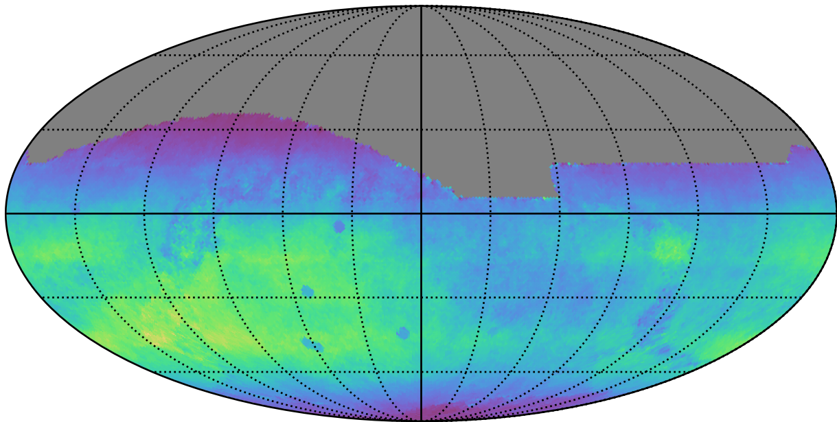
too_100_4v3.4_10yrs All sky r band: Normalized Teff
