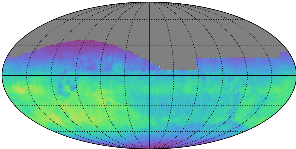
too_100_4v3.4_10yrs All sky i band: Normalized Teff
