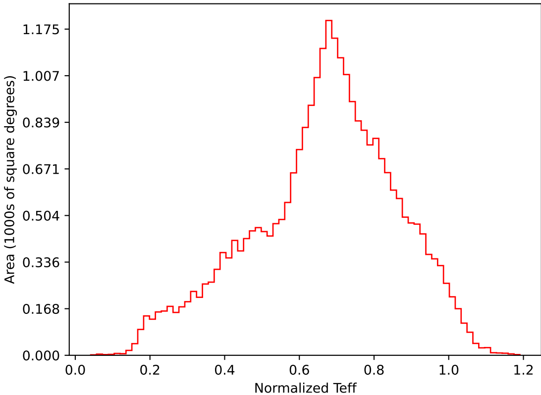
too_100_4v3.4_10yrs All sky i band: Normalized Teff
