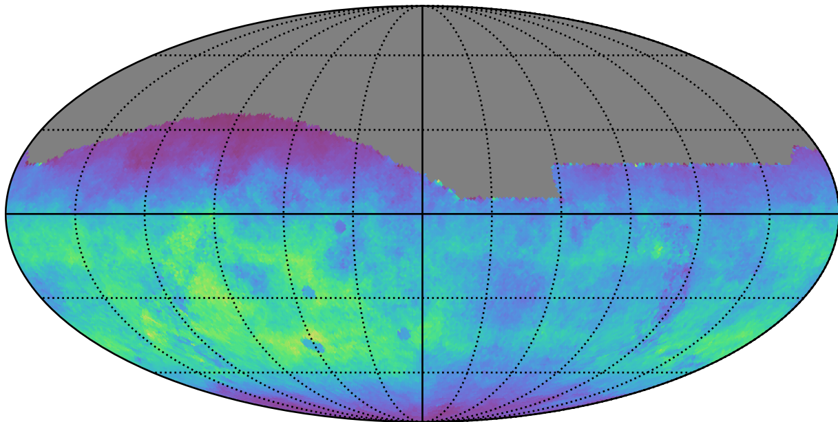
too_100_4v3.4_10yrs All sky g band: Normalized Teff
