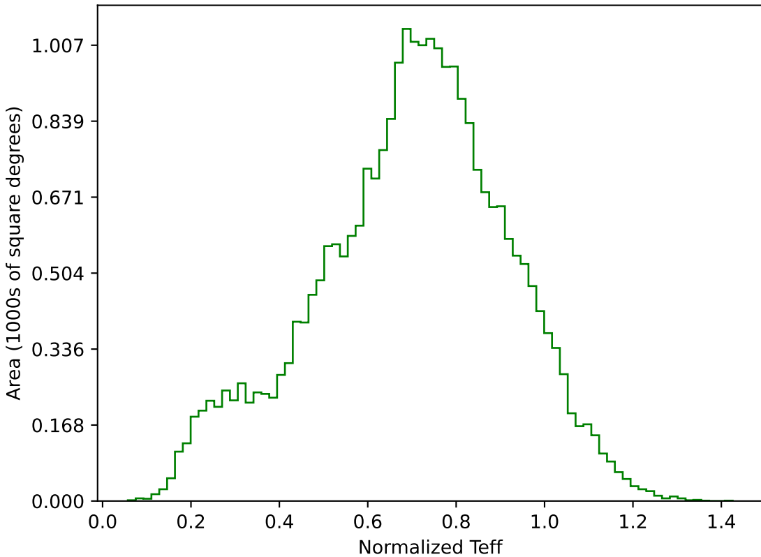
too_100_4v3.4_10yrs All sky g band: Normalized Teff
