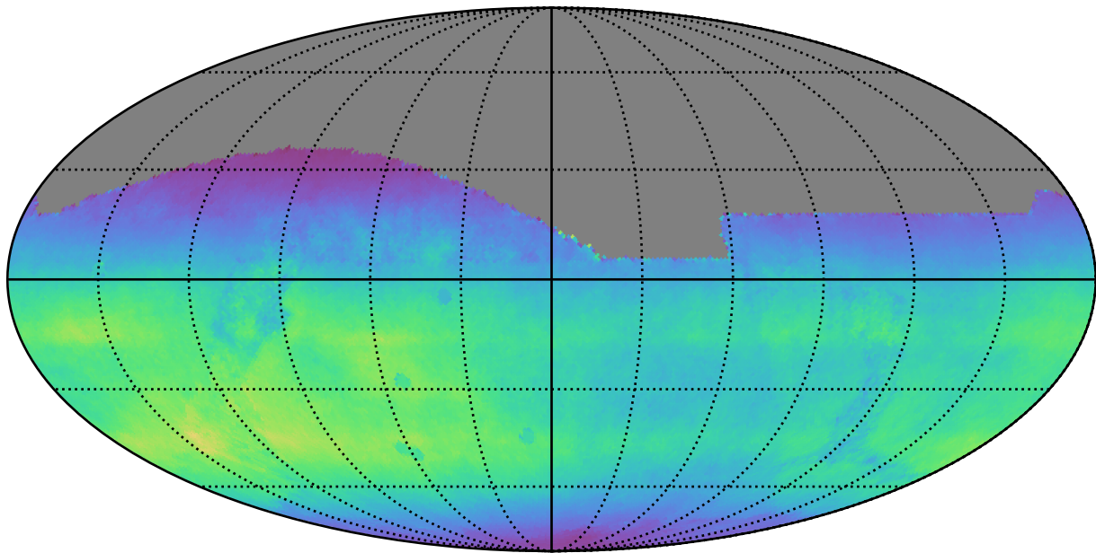
too_100_4v3.4_10yrs All sky all bands: Normalized Teff
