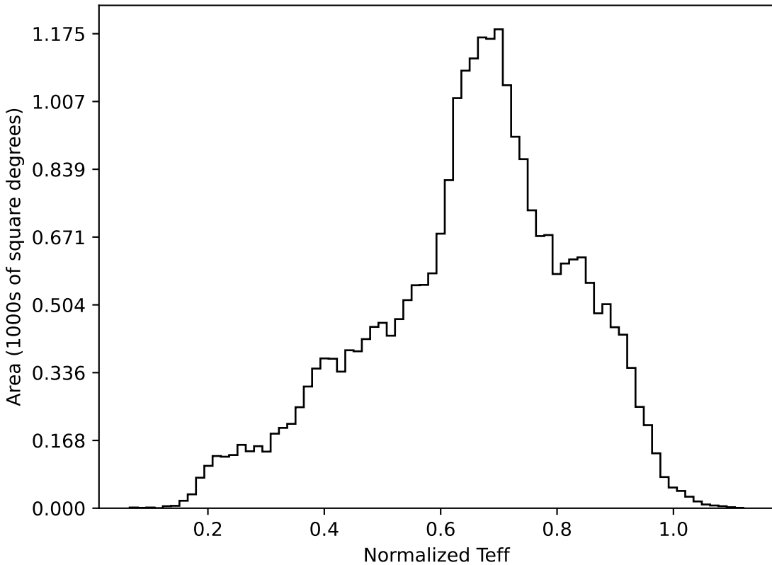
too_100_4v3.4_10yrs All sky all bands: Normalized Teff
