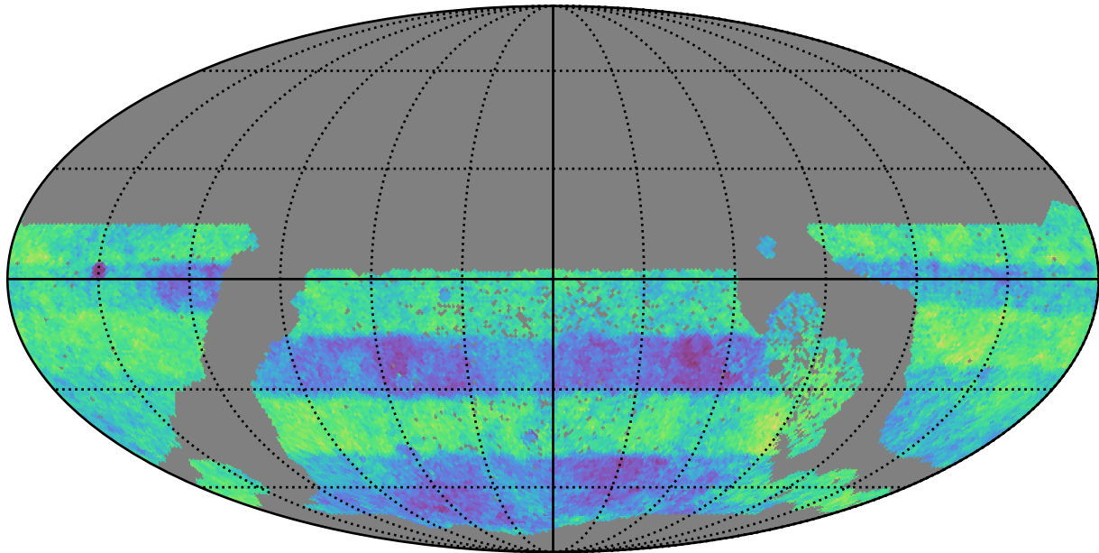
too_100_4v3.4_10yrs WFD: Normalized Proper Motion Uncert @ 24.0
