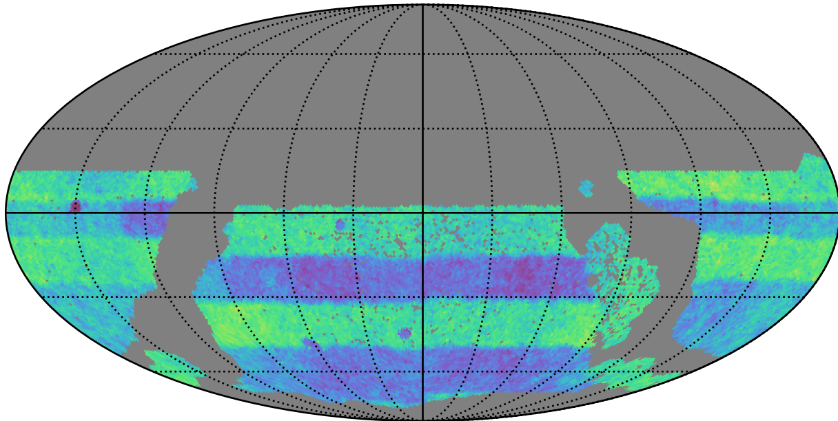
too_100_4v3.4_10yrs WFD: Normalized Proper Motion Uncert @ 20.5
