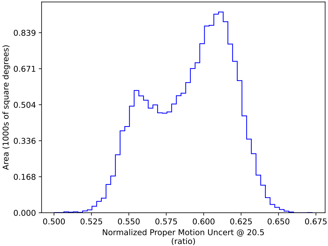
too_100_4v3.4_10yrs WFD: Normalized Proper Motion Uncert @ 20.5
