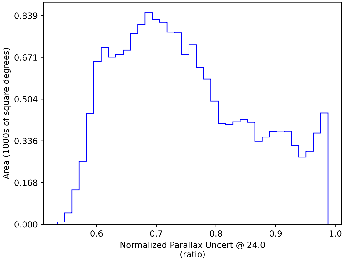
too_100_4v3.4_10yrs WFD: Normalized Parallax Uncert @ 24.0
