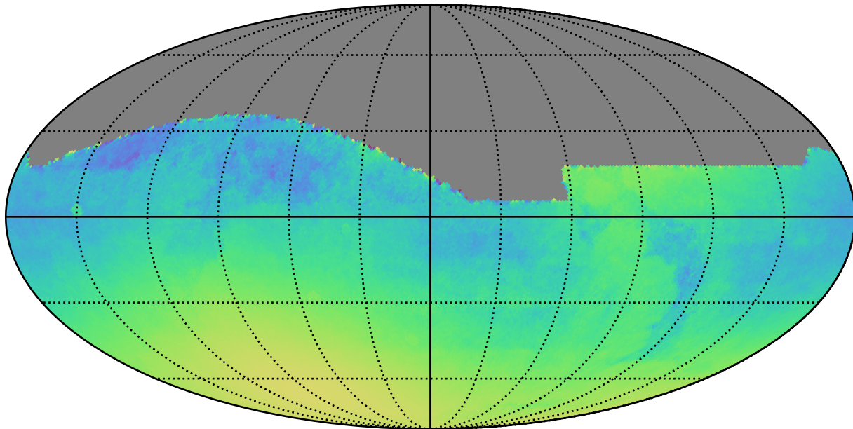
too_100_4v3.4_10yrs All sky: Normalized Parallax Uncert @ 24.0
