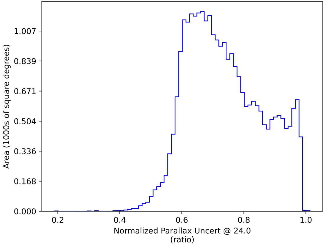
too_100_4v3.4_10yrs All sky: Normalized Parallax Uncert @ 24.0
