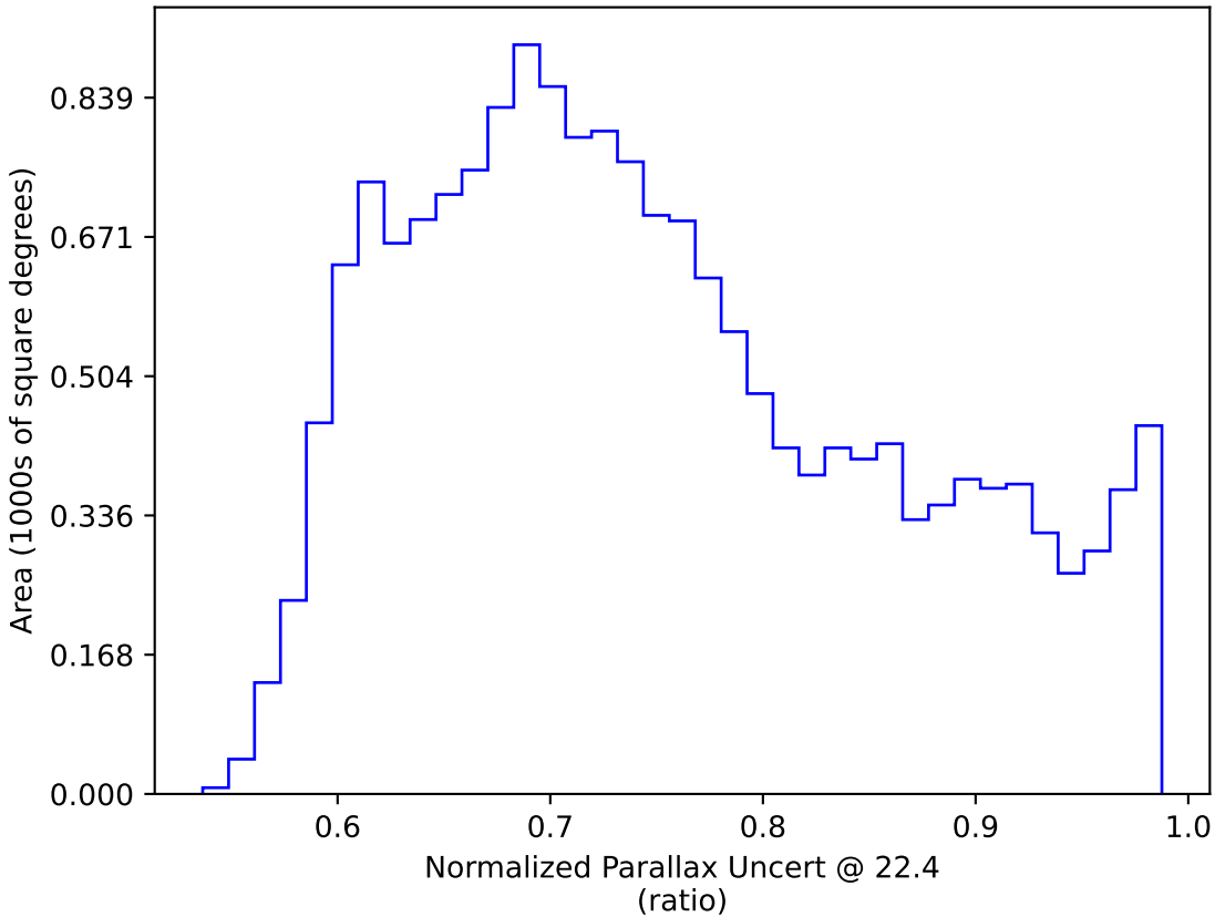
too_100_4v3.4_10yrs WFD: Normalized Parallax Uncert @ 22.4
