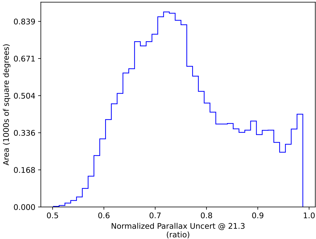
too_100_4v3.4_10yrs WFD y band only: Normalized Parallax Uncert @ 21.3
