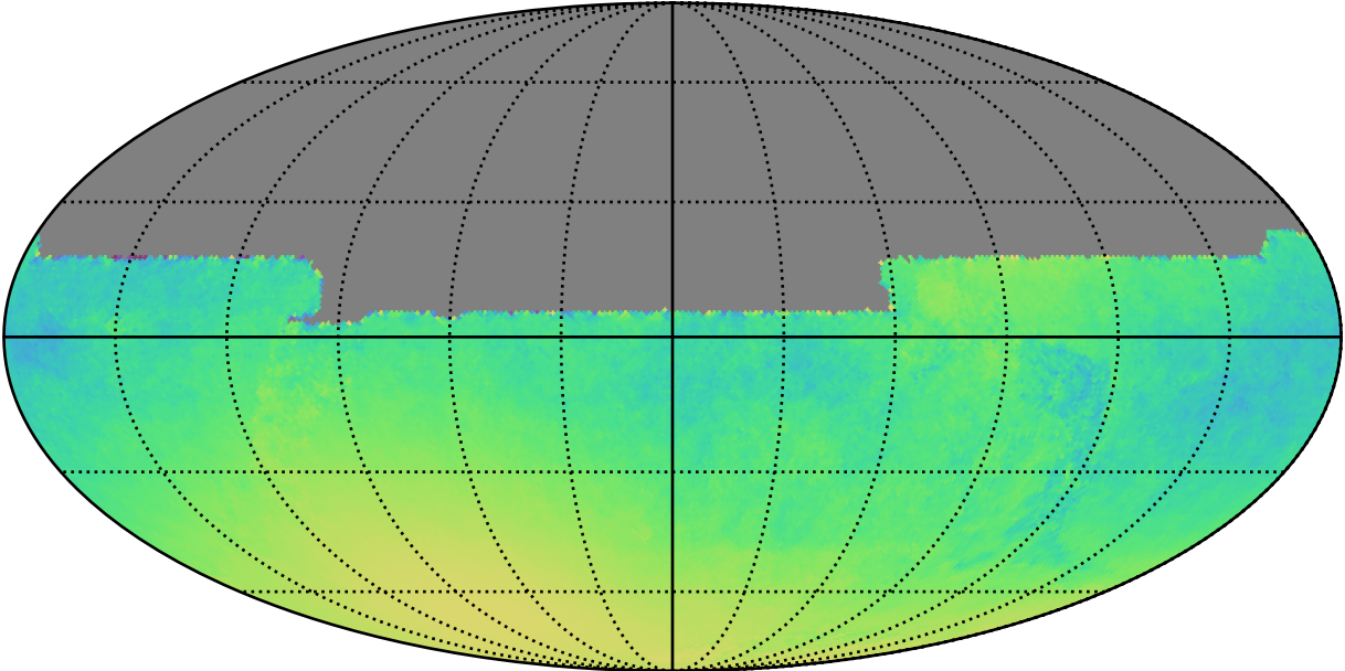
too_100_4v3.4_10yrs All sky y band only: Normalized Parallax Uncert @ 21.3
