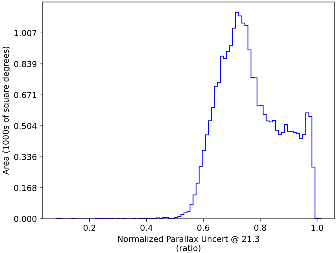
too_100_4v3.4_10yrs All sky y band only: Normalized Parallax Uncert @ 21.3
