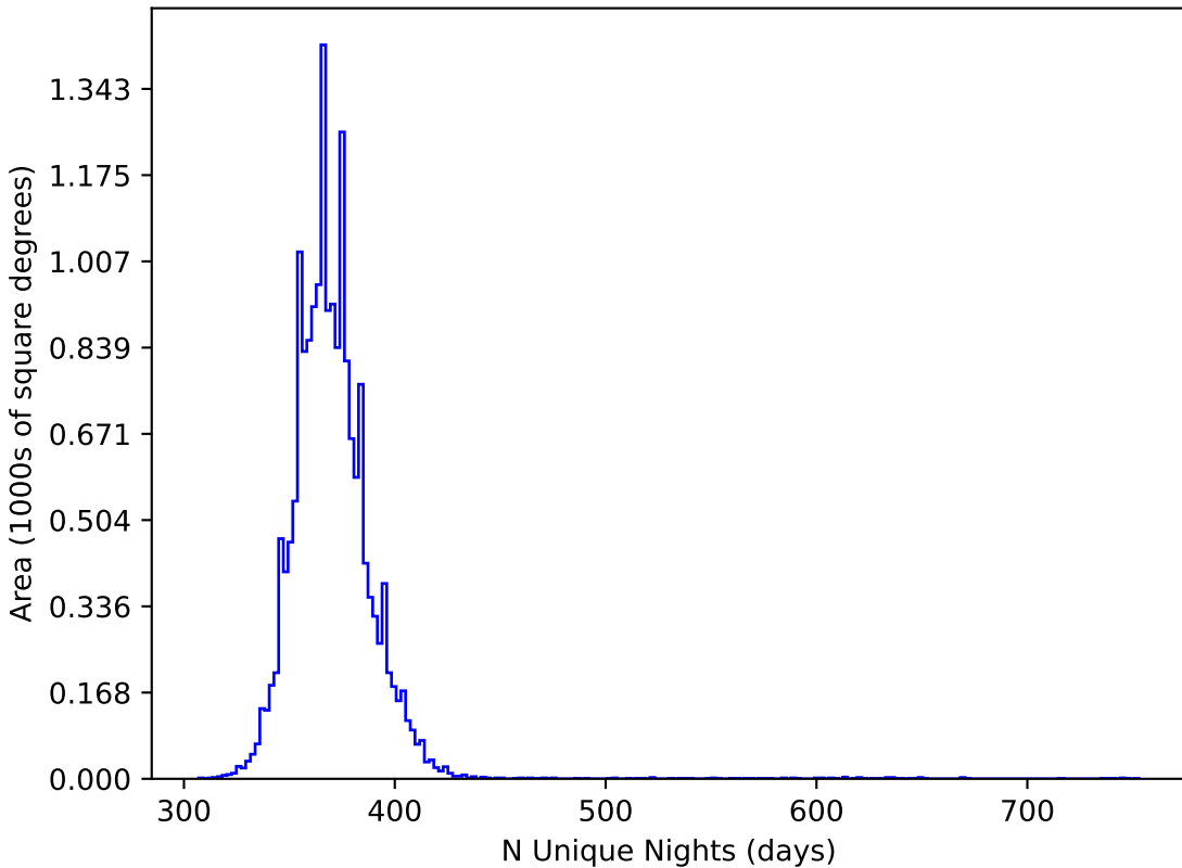
too_100_4v3.4_10yrs WFD all bands: N Unique Nights
