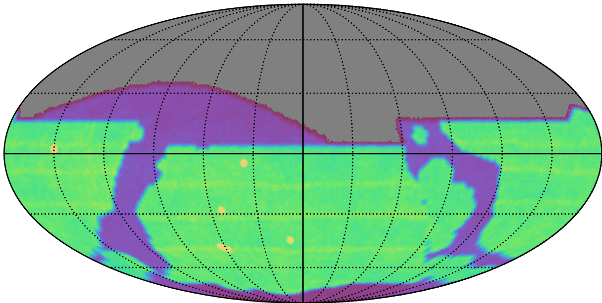
too_100_4v3.4_10yrs All sky all bands: N Unique Nights
