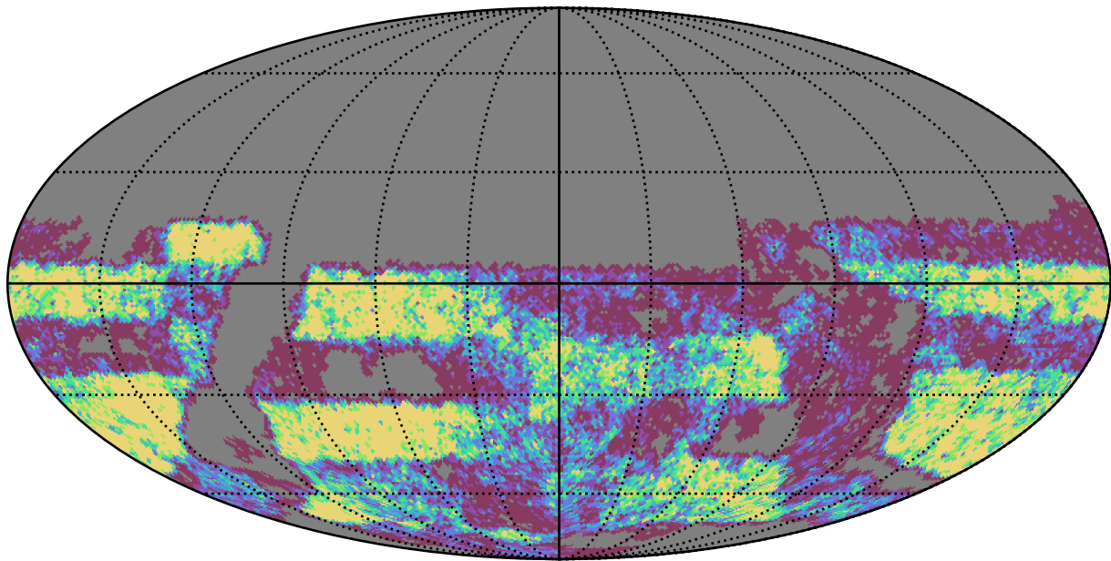
too_100_4v3.4_10yrs Yr 3-4 u band: NVisits
