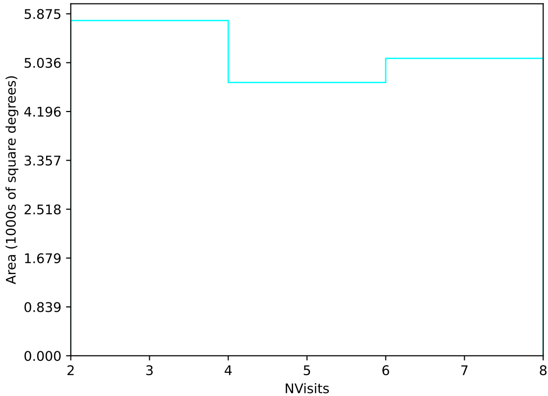
too_100_4v3.4_10yrs Yr 3-4 u band: NVisits
