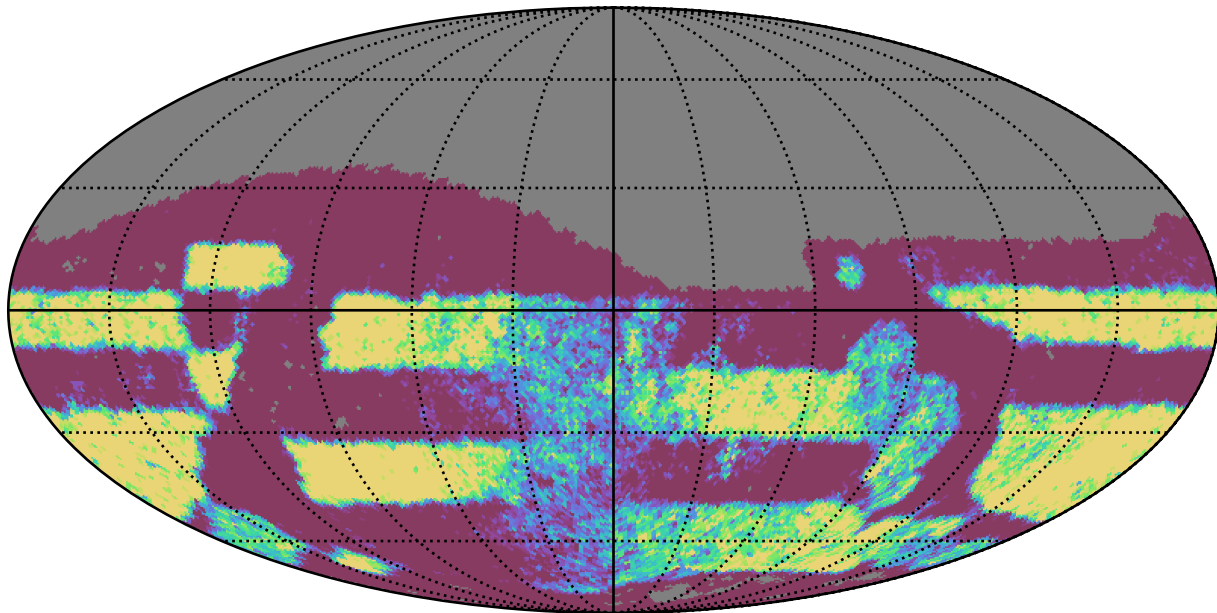
too_100_4v3.4_10yrs Yr 3-4 r band: NVisits
