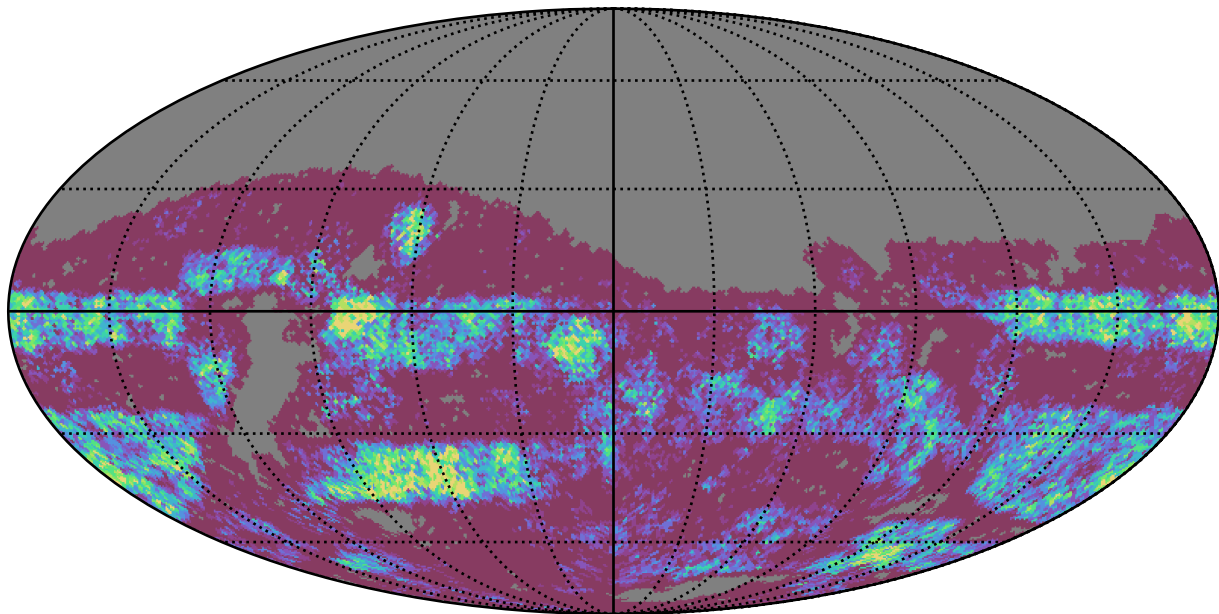
too_100_4v3.4_10yrs Yr 3-4 g band: NVisits
