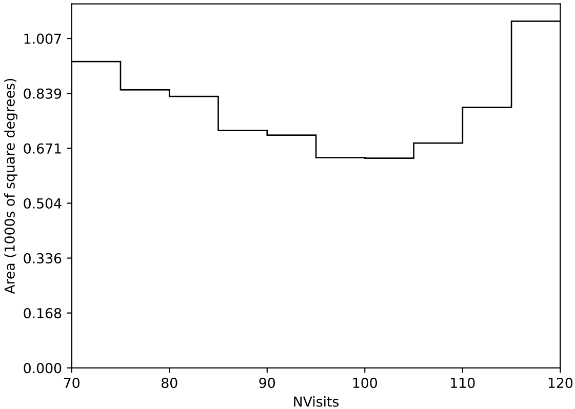
too_100_4v3.4_10yrs Yr 3-4 all bands: NVisits
