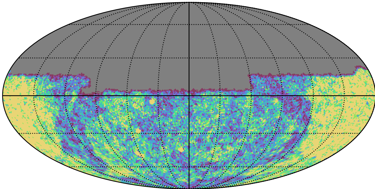
too_100_4v3.4_10yrs Yr 1 u band: NVisits
