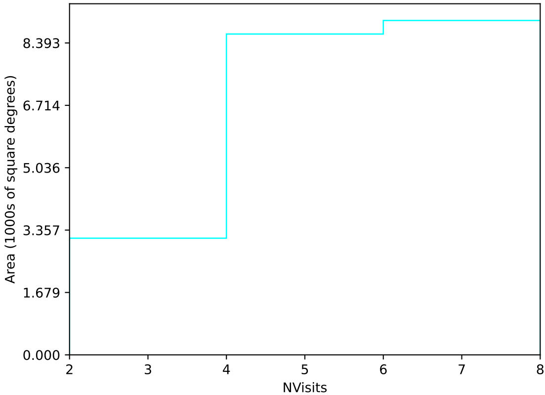
too_100_4v3.4_10yrs Yr 1 u band: NVisits
